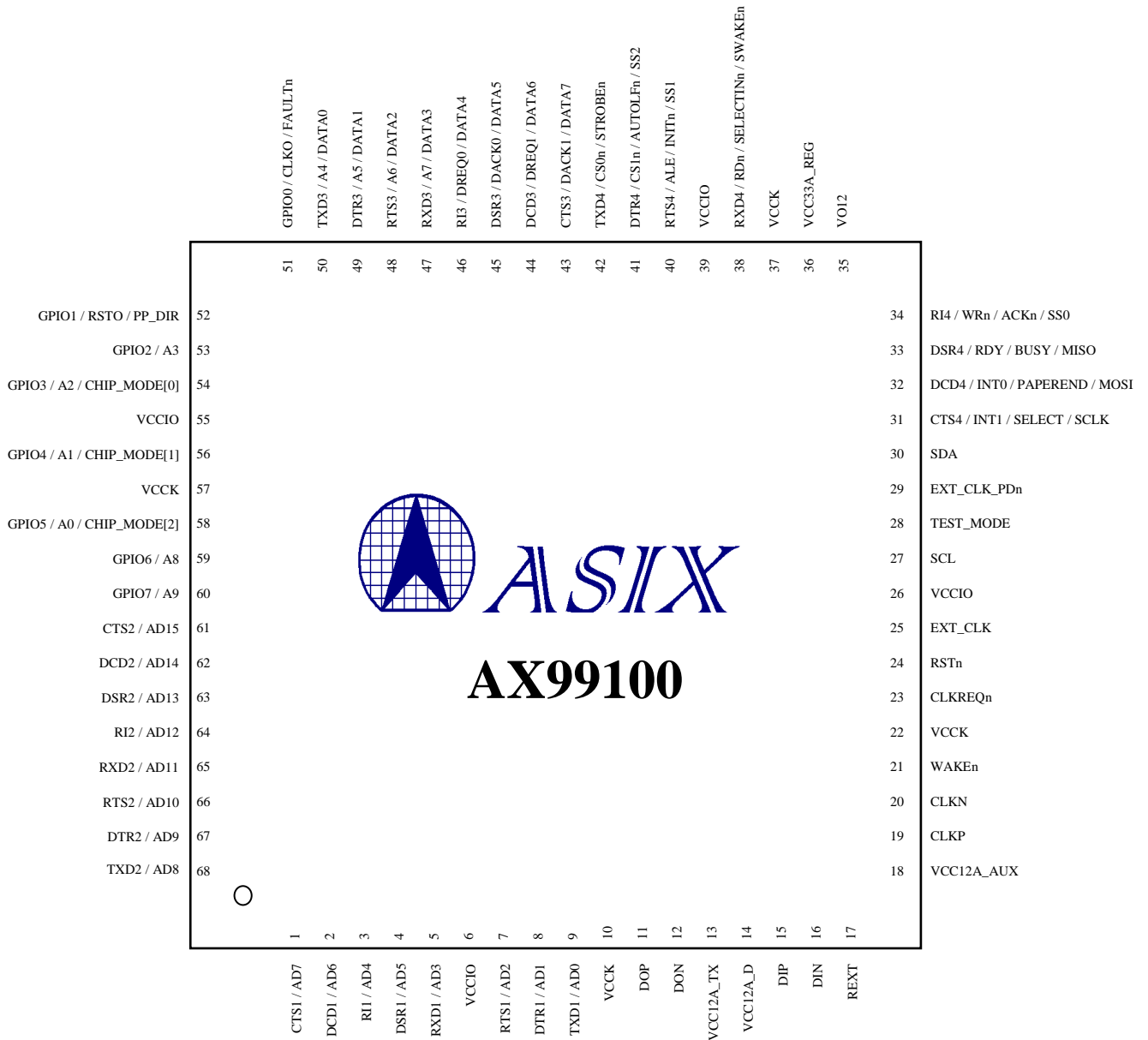
Figure 1-2: AX99100 Pinout Diagram
