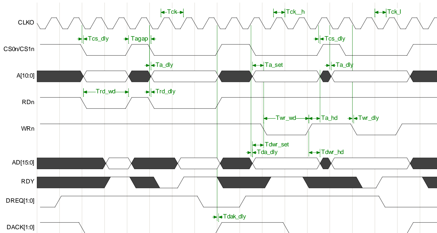
Figure 4-3: Non-multiplexed Bus Type with External RDY Timing Diagram
